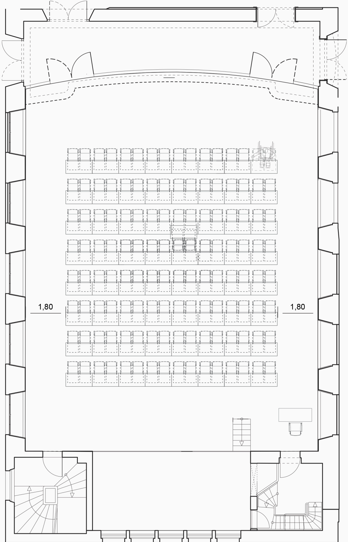
Goethe Hall 251,22m 2 max. 128 persons M.1:100
