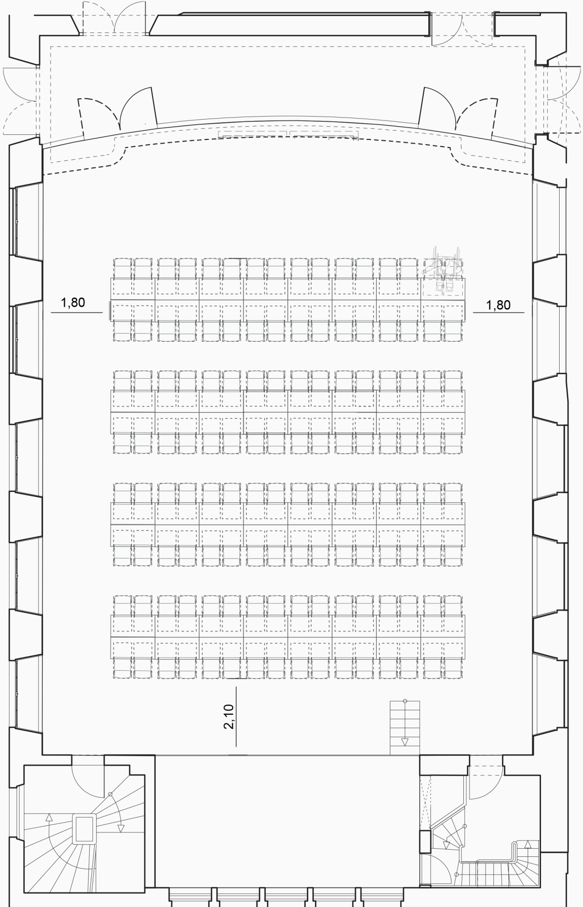
Goethe Hall 251,2m 2 max. 128 persons M,1:100
